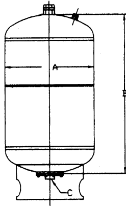
12 GAL. THRU 37 GAL. FACTORY PRE-CHARGE 40PSI
