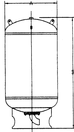
45 GAL. THRU 132 GAL. FACTORY PRE-CHARGE 55PSI
