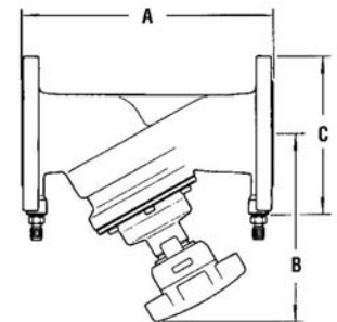
Flanged Model
